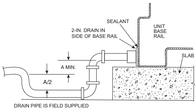
Primary Condensate Drain Piping Details (Slab and Curb Mounted) and Secondary Condensate Drain Piping Details (Slab-Mounted)
